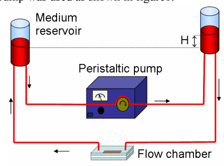
Figure 1. Steady laminar flow setup
